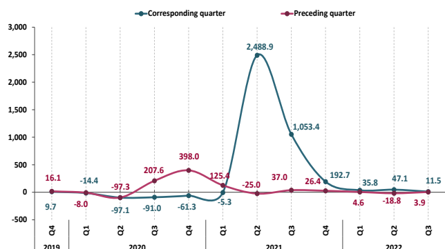
Figure 6: Tourist bed-nights
