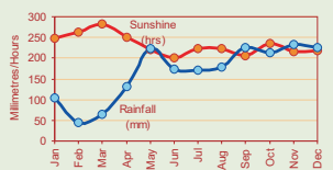
28 YEARS AVERAGE OF MONTHLY SUNSHINE & RAINFALL (MALE), 1975 - 2004
