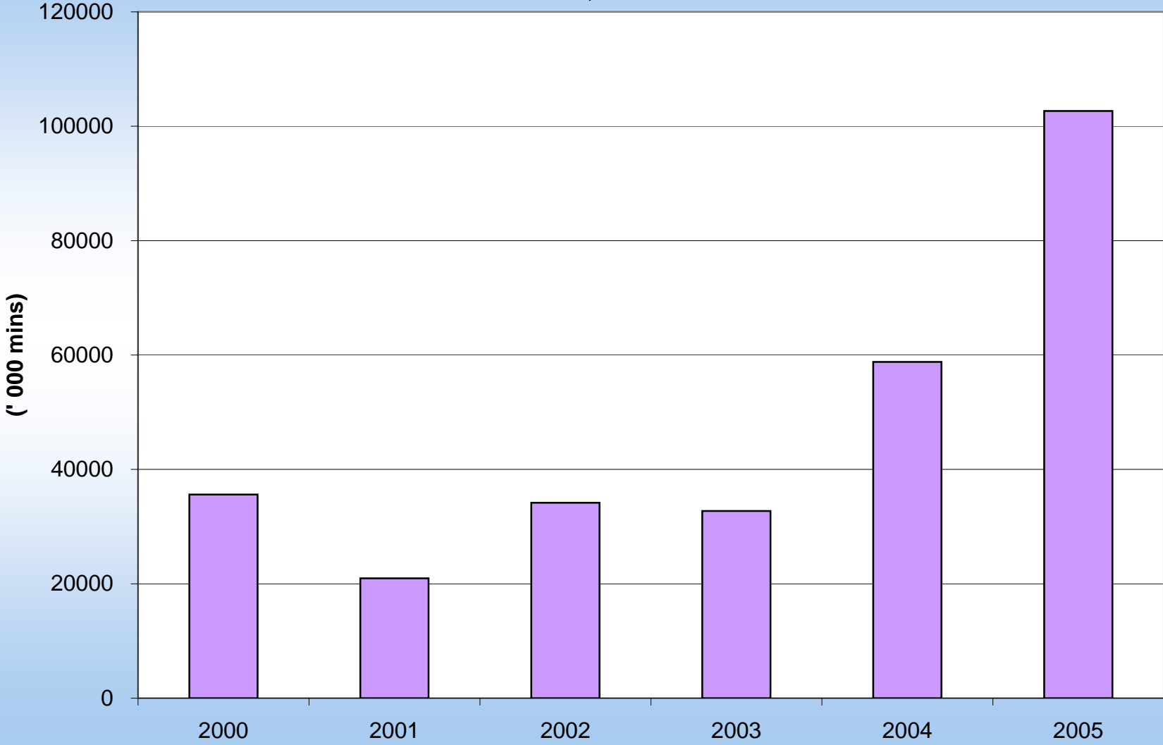
FIG 11.6: MOBILE CALLS, 2000-2005
