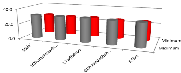
Yearly Average of daily maximum and minimum temperature, 2013 (degree celcius)
